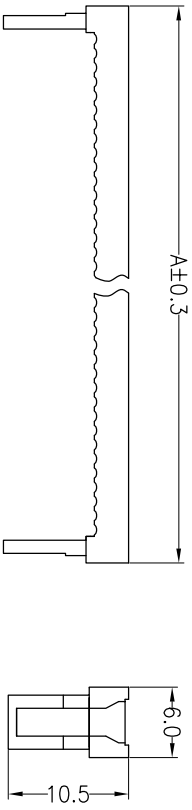
Strain relief P/N:G5315-XXDB01
